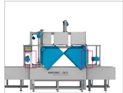
Openings in the carrier system for belt body replacement
